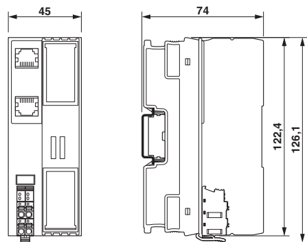
Dimensional drawing
